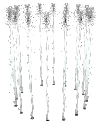
AQUA CAGE GPM: 50 Height Adjustable Water Depth: 0 - 1" All 304 SS Construction
